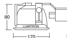
LMDL-8B Cut-out 150mm.
