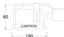
LMDL-8C Cut-out 170mm.
