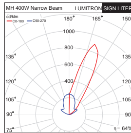
SL-400MH-T Narrow Beam
