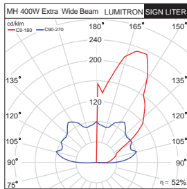
SL-400MH-T Extra Wide Beam
