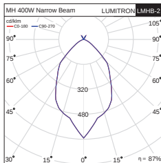
Narrow Beam
