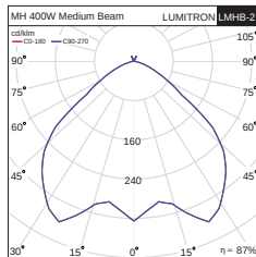
Medium Beam
