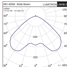
Wide Beam
