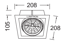
Cut-out 160x160mm.
