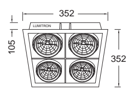
Cut-out 312x312mm.
