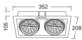
Cut-out 160x312mm.
