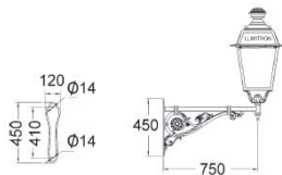
Wall Mount Version
